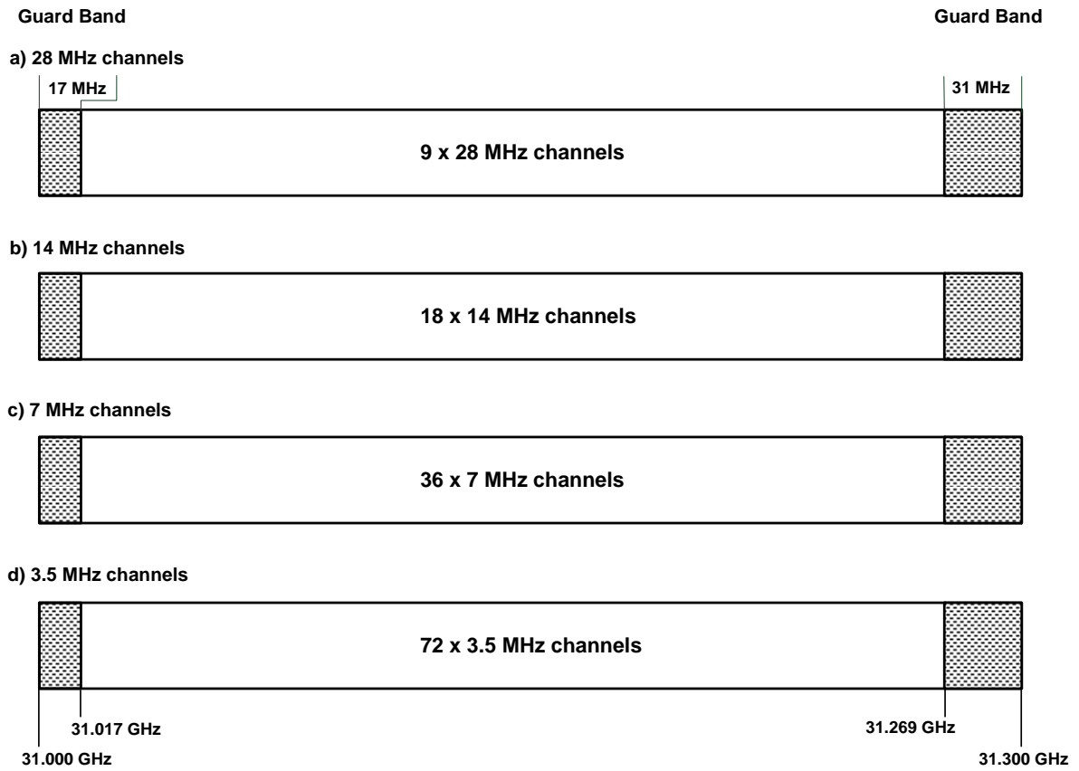
Figure A1: Occupied spectrum: 31.0 to 31.3 GHz Band for TDD systems
