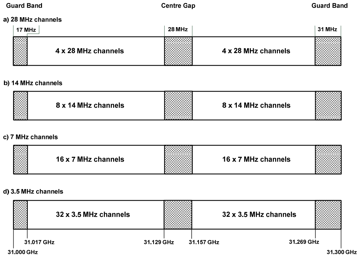
Figure B1: Occupied spectrum: 31.0 to 31.3 GHz Band for FDD systems
